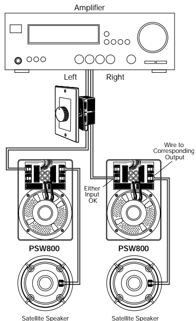
Figure 4 A Single PSW800 Hook-Up
